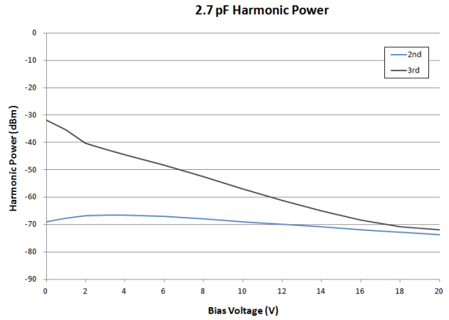
Figure 2. Harmonic Power
